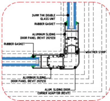
DETAIL-3
