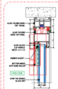
SECTION - A
