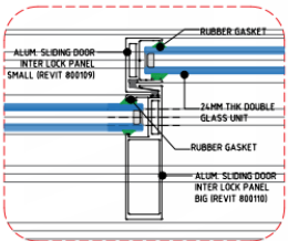
DETAIL-2
