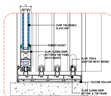
SECTION - A
