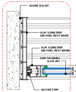
DETAIL-1
