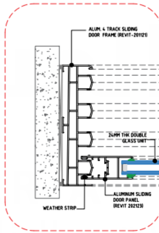
DETAIL-1
