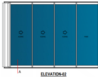
ELEVATION-02 SCALE 1:50
