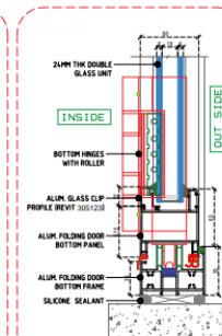
SECTION - B
