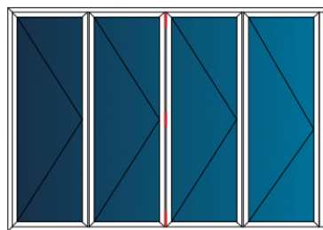
ELEVATION-01 SCALE 1:50
